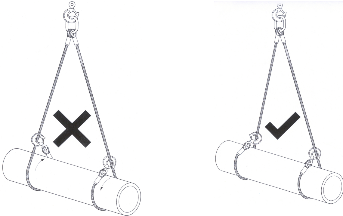
Figure A.2 — Choke hitches (continued)
