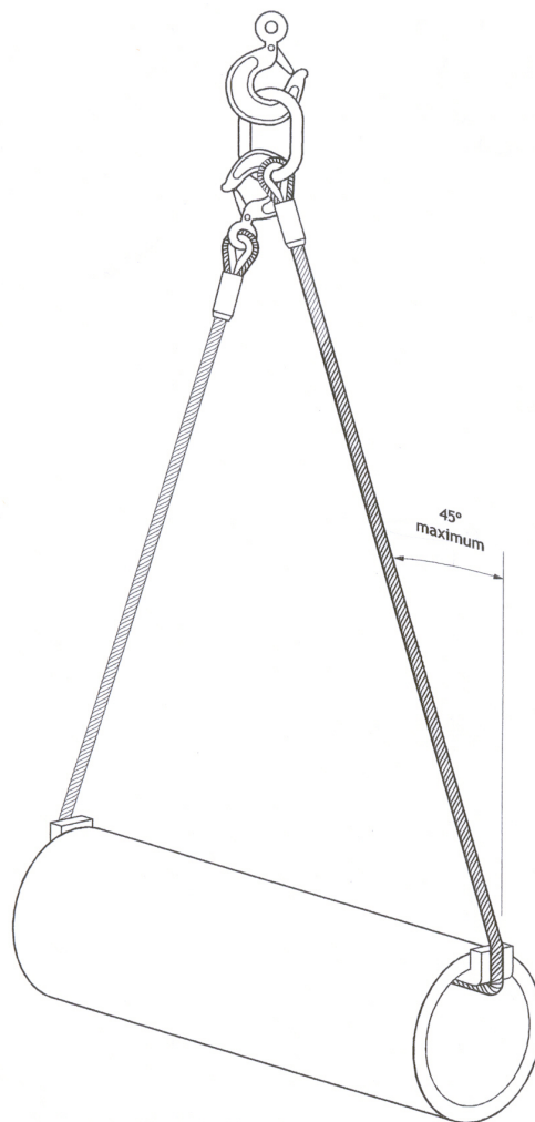
Figure A.4 — Basket hitches
